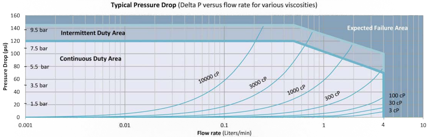
G015 / G015HZ Pressure Drop Graph
